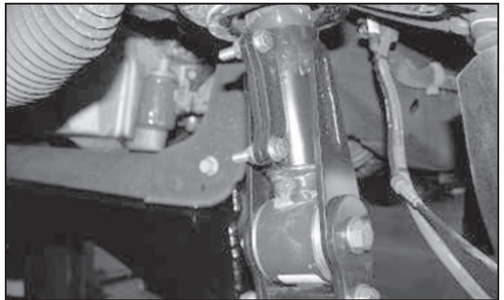
FIGURE 42 - STEP 31
