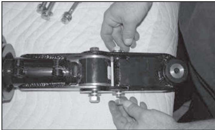
FIGURE 39 - STEP 30
