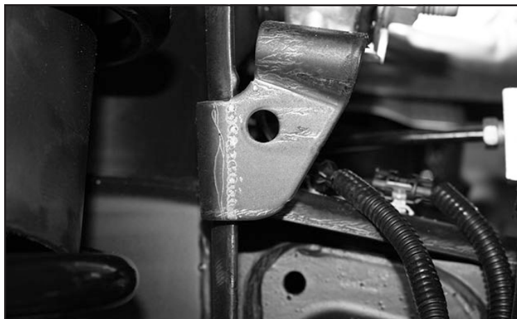
FIGURE 12 - STEP 11
