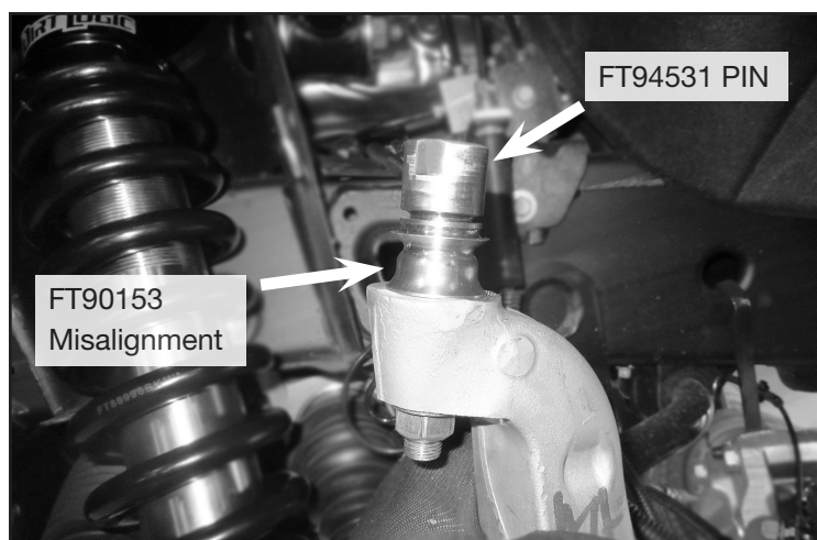
FIGURE 15 - STEP 13
