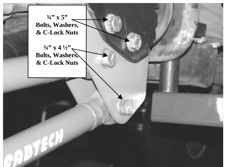
Assembly of the FT292 Alignment Cam
