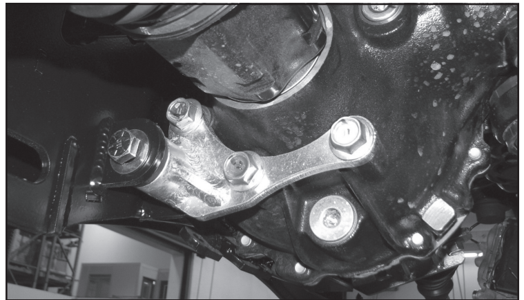
FIGURE 19 - STEP 24
