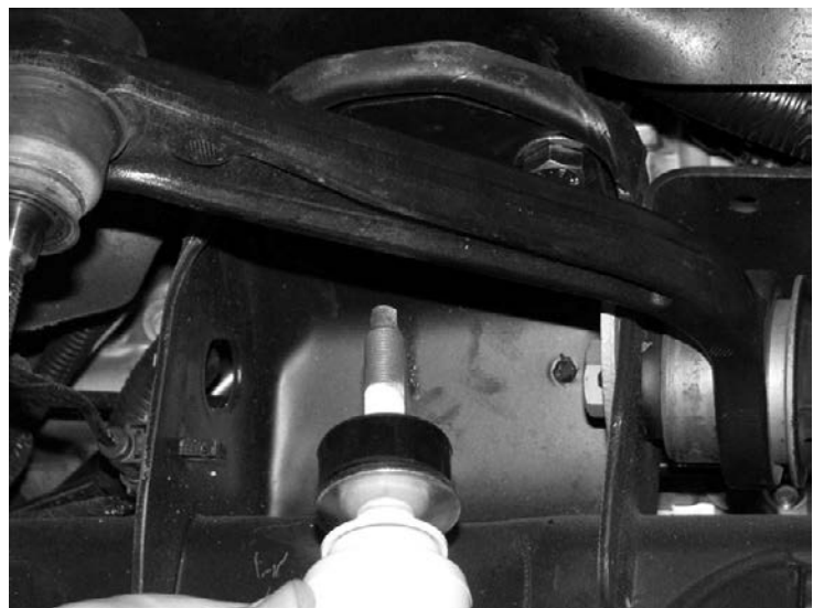
38. Install the front shock (FTS7338) or (FTS6338) with the stem in the upper mount. SEE PHOTOS BELOW
