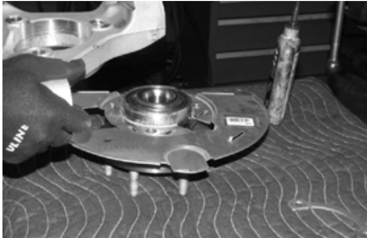
FIGURE 65 - STEP 41
