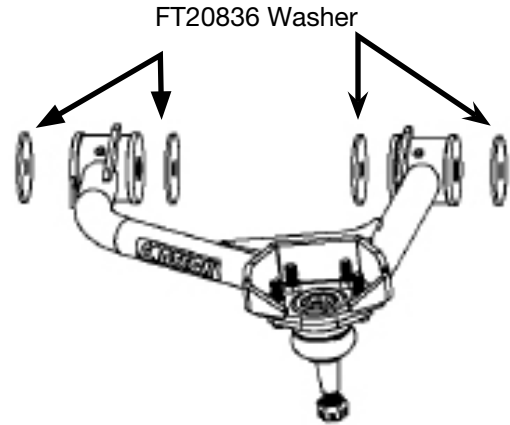
FIGURE 35 - STEP 26
