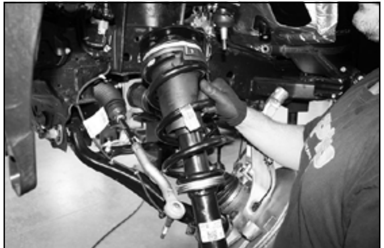
FIGURE 36 - STEP 28
