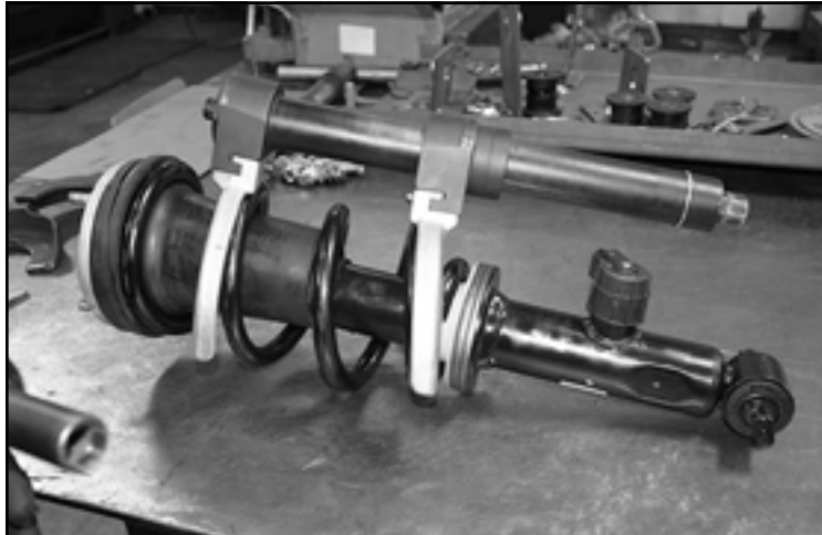
FIGURE 21 - STEP 16
