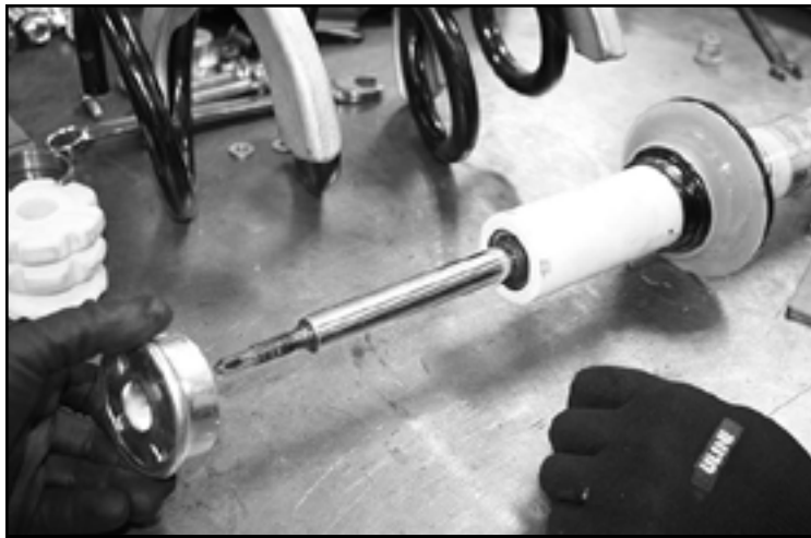
FIGURE 16 - STEP 12
