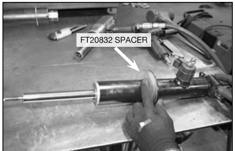
FIGURE 25 - STEP 18
