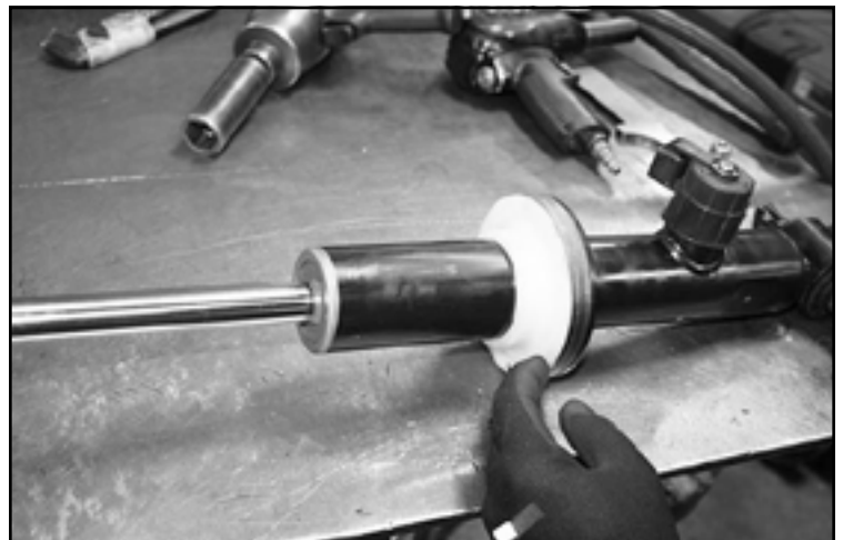
FIGURE 26 - STEP 18
