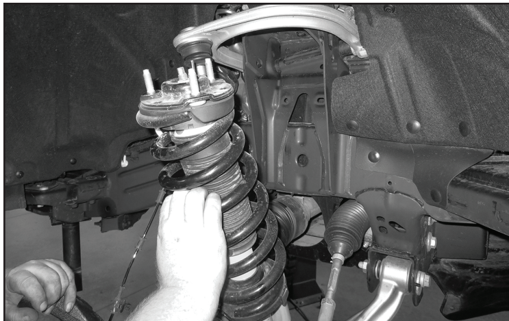
FIGURE 9 - STEP 7
