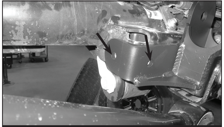
FIGURE 26 - STEP 40
