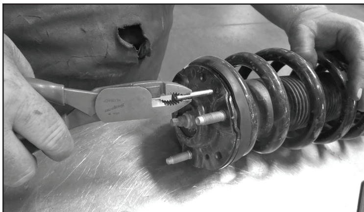
FIGURE 10 - STEP 10
