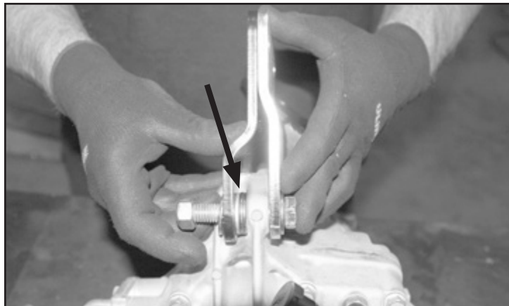
FIGURE 14 - STEP 24
