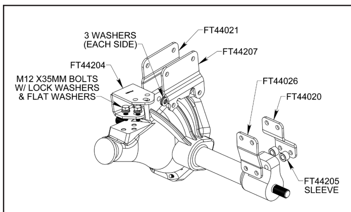
FIGURE 16 - STEP 23 - 25
