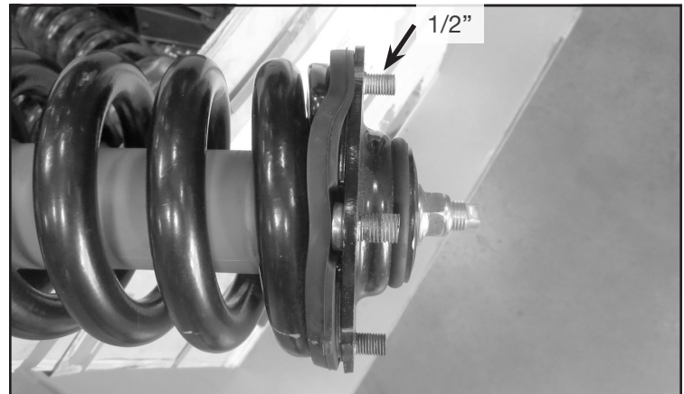
FIGURE 7 - STEP 12
