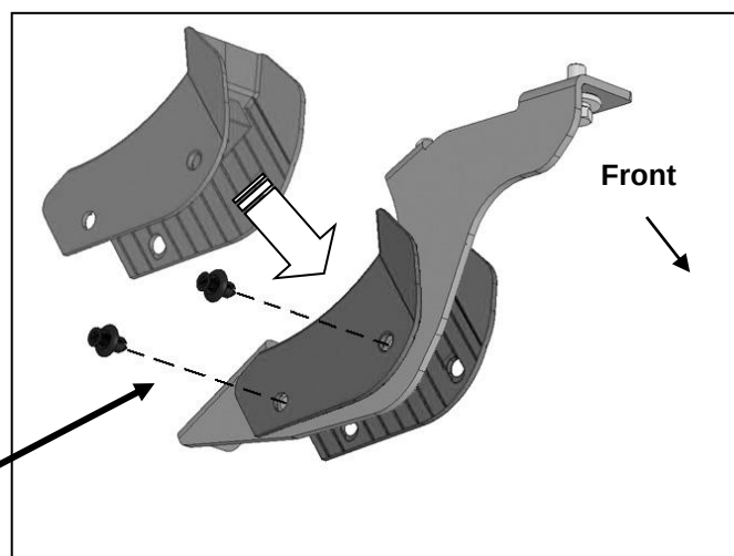
(Fig 4) Attach Plastic Cover to Bracket
