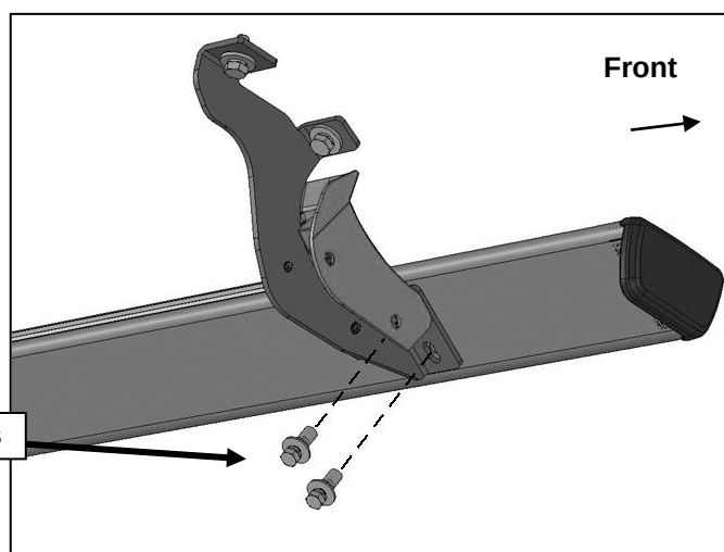
(Fig 8) Attach Driver/Left Sidebar to Mounting Brackets (Driver/left front illustrated)
