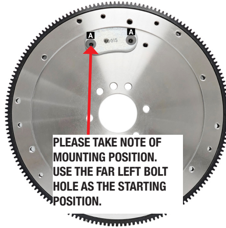
1630583 W/6001S COUNTERWEIGHT
